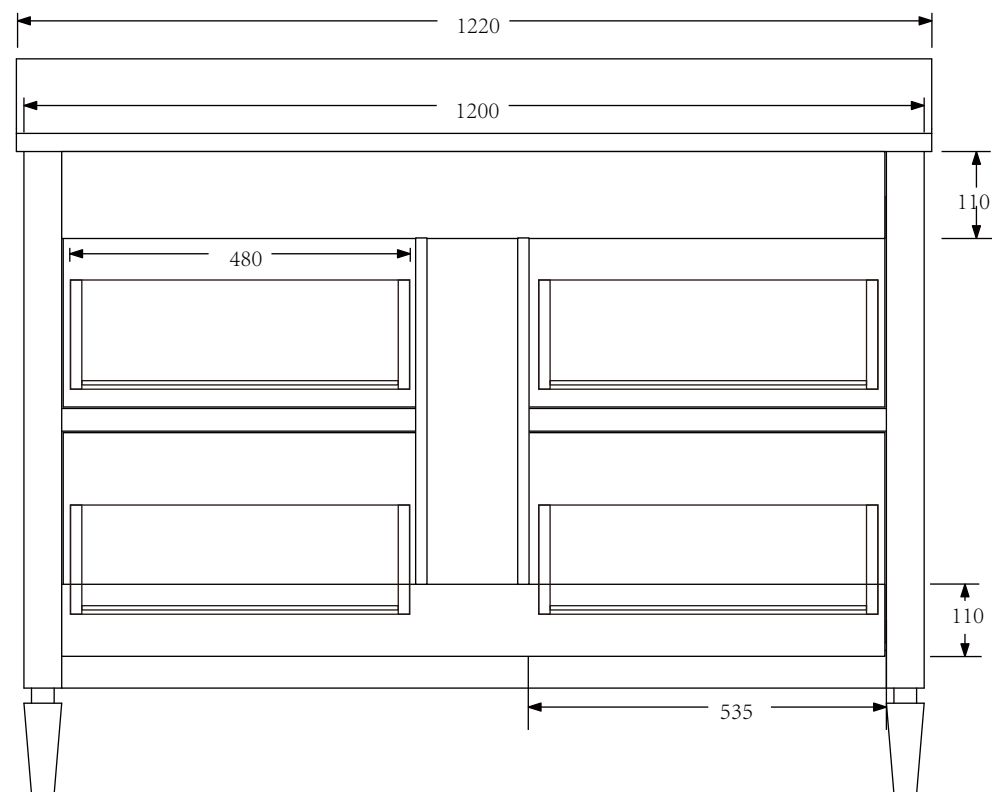
Back View
